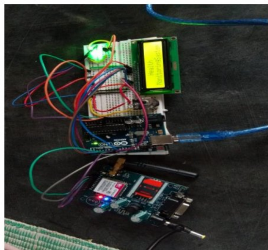
Figure 8. Hardware Setup
