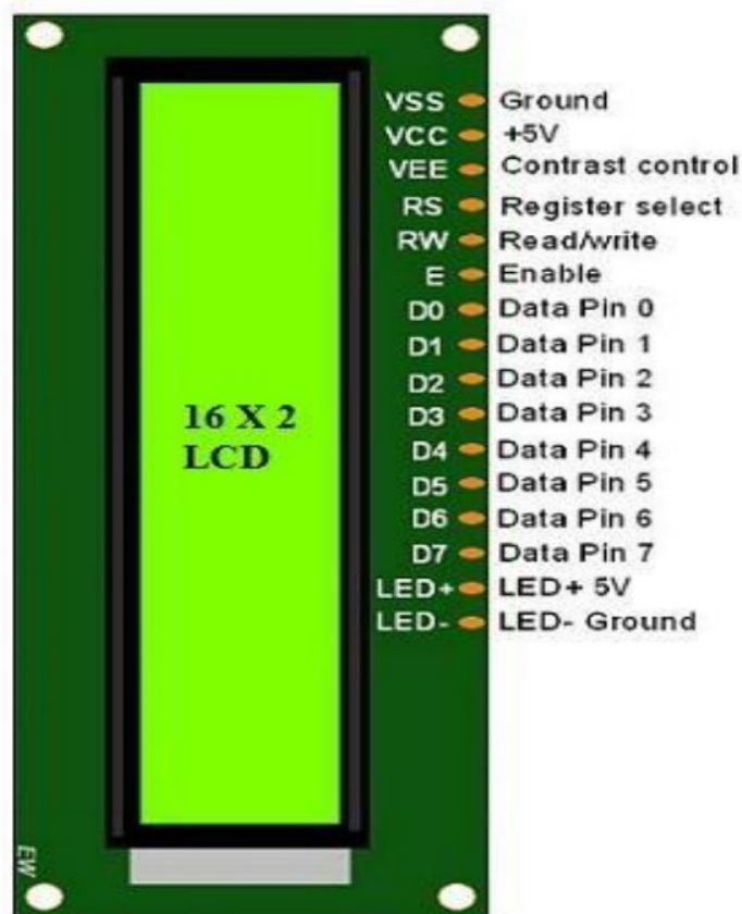
Figure 3.6 Pin diagram of LCD
