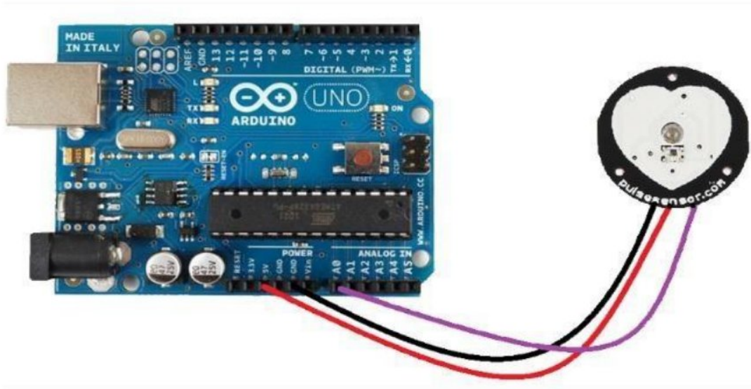
Figure3.5: Interfacing of pulse sensor with Arduino
