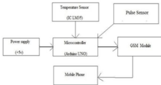
Figure 2. Block Diagram of Remote health monitoring system
