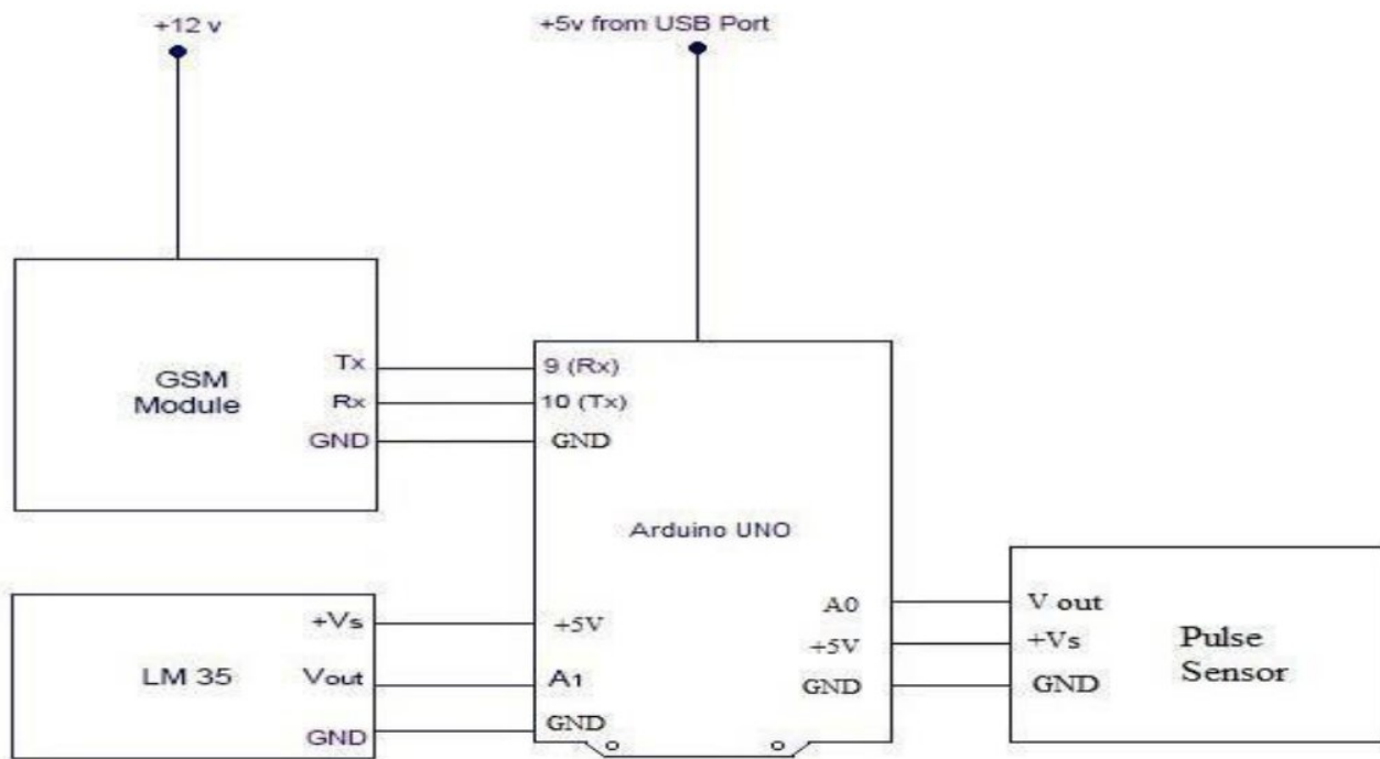
Figure 4.2: Circuit Diagram of proposed system
