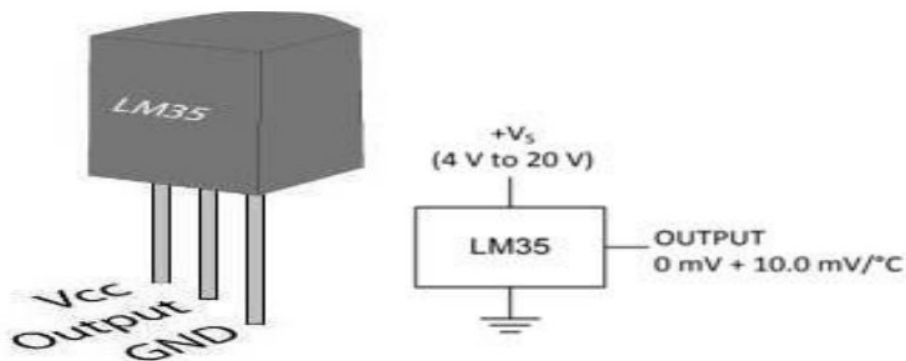
Figure 3.2: LM35 Temperature sensor
