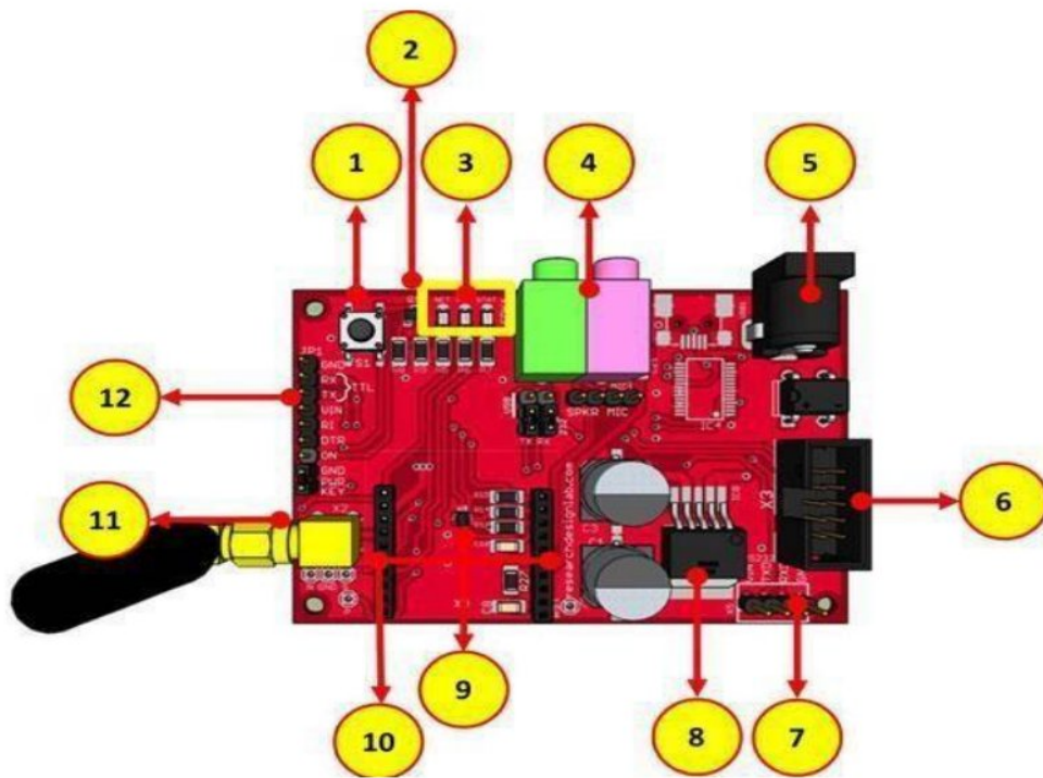
Figure 3.3: GSM Module
